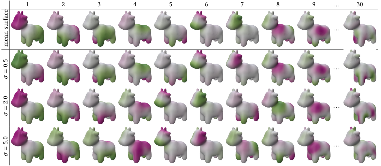
Fig. 5. We show the eigenfunctions associated to the smallest 9 eigenvalues of the cotan Laplacian of the mean surface (first row) and of our M_\varphi^{-1}L_\varphi operator (also the 30th) on the mean surface for various sigma \sigma values and h = 1/200 .
